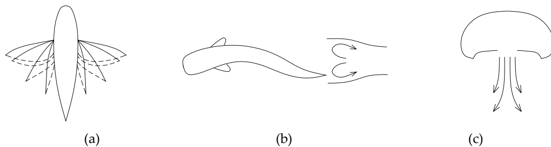
Figure 2. Main propulsion procedures from the view point of hydrodynamics; (a) Drag-based; (b) Added mass; (c) Momentum injection.
