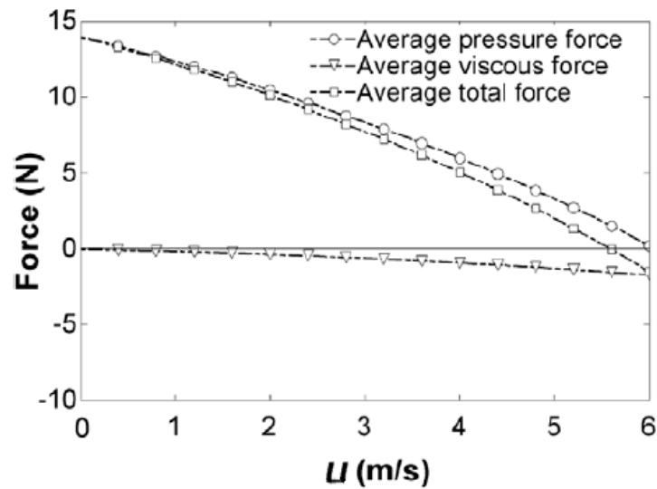
Figure 6. Average forces against cruising velocity for anguilliform swimming [50].
