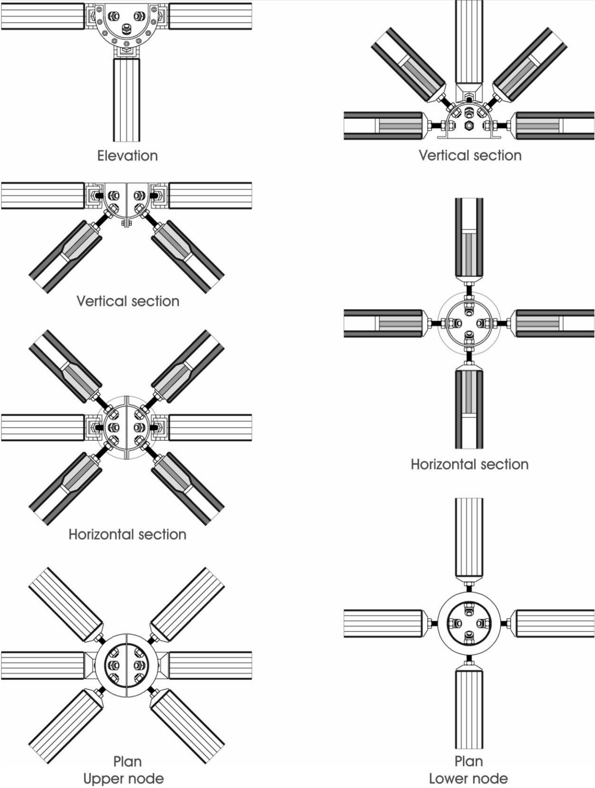
Figure 13: Nodes
