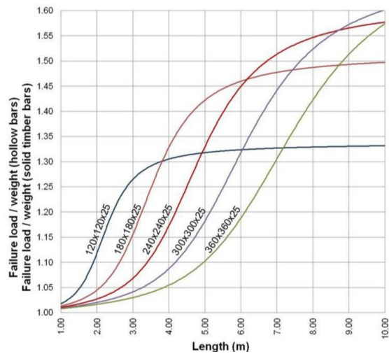
Figure 1: Hollow bars Figure 2: Comparative performance: hollow bars versus solid section bars
