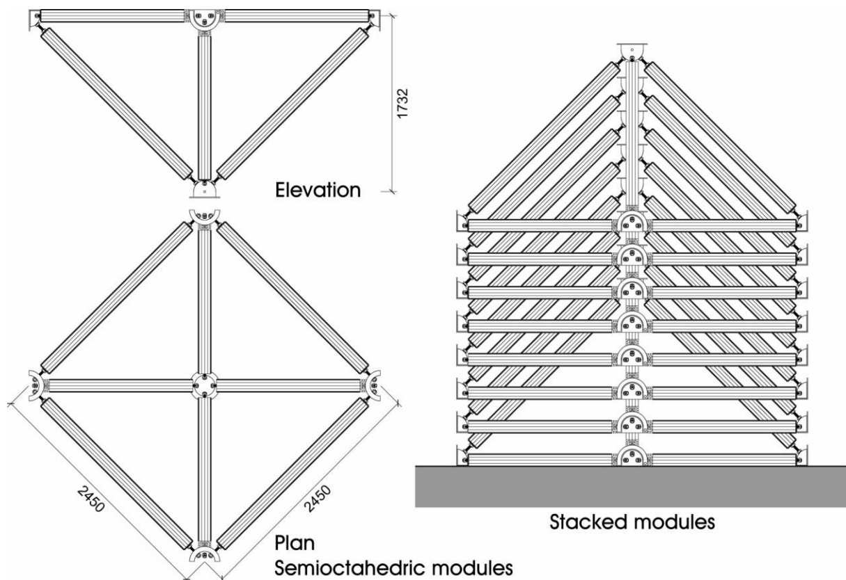
Figure 12: Stackable modules
