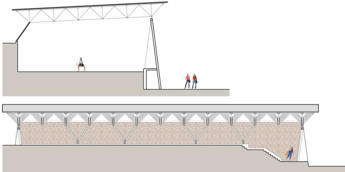
Figure 7: Sections
