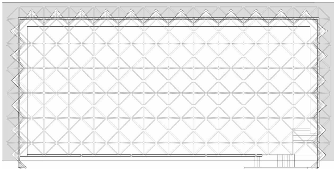
Figure 8: Plan
