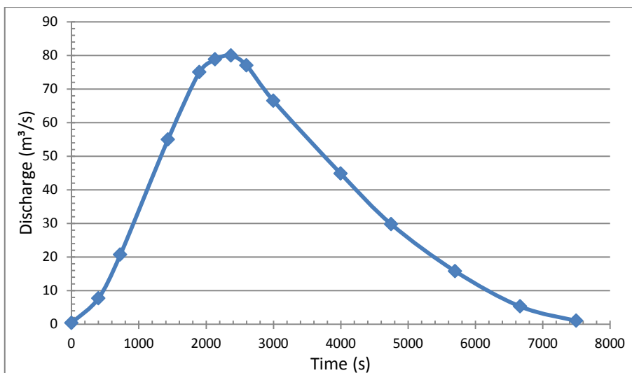
Figure 23. Hydrograph of standard project flood for a return period of 500 years.
