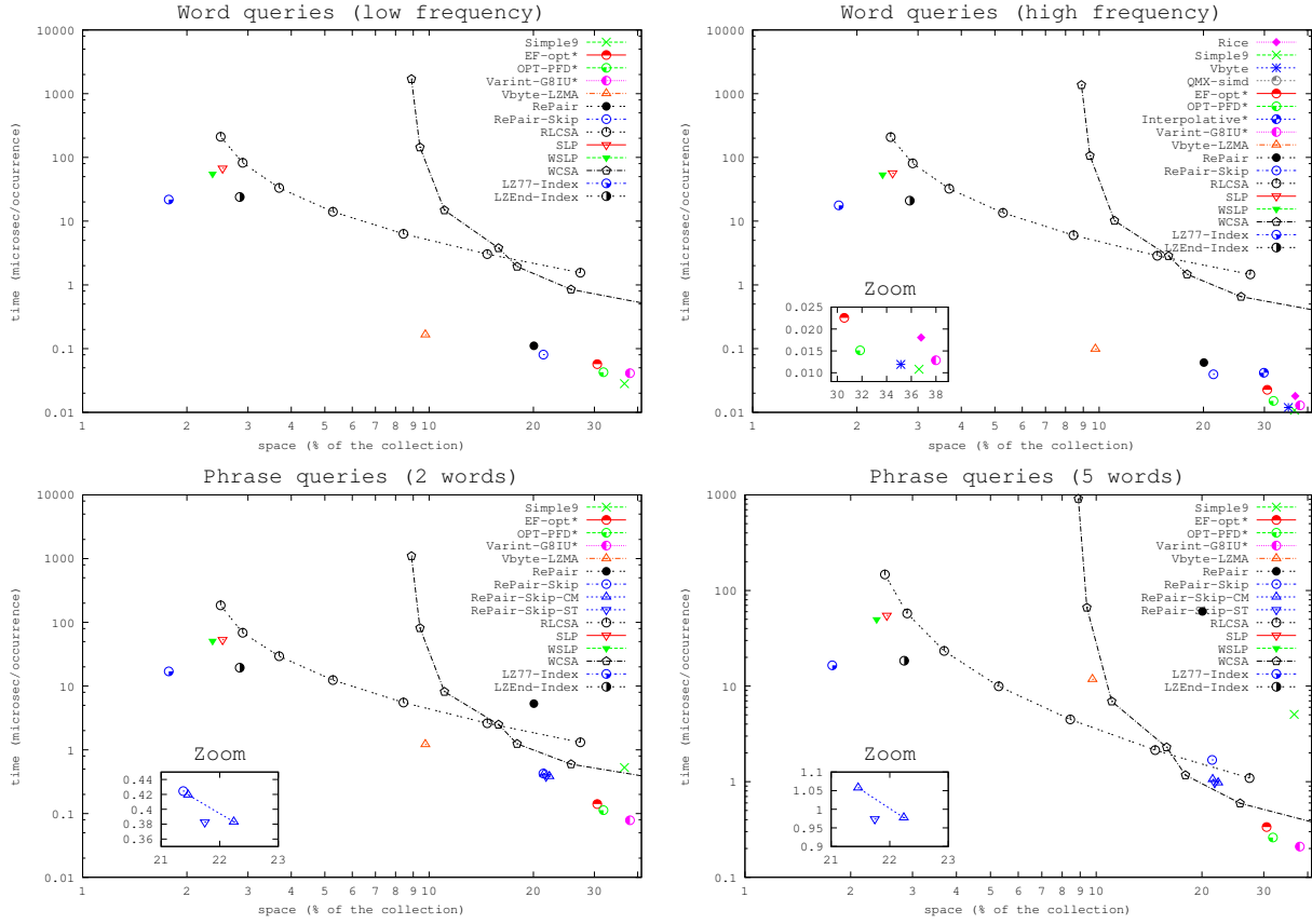
Figure 9: Space/time tradeoffs for positional indexes. Logscale.
