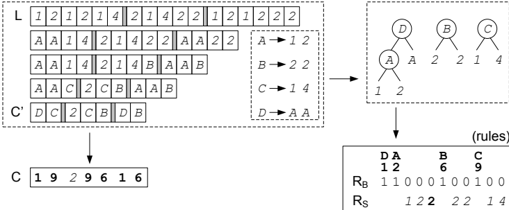
Figure 1: Example of Re-Pair compression. Solid boxes ( C and rules ) enclose the data represented. Bold numbers (nonterminals) in the final C sequence and R_S refer to positions in R_B , whereas slanted ones (terminals) refer to original values. To distinguish them, the maximum offset u is added to the bold numbers.
