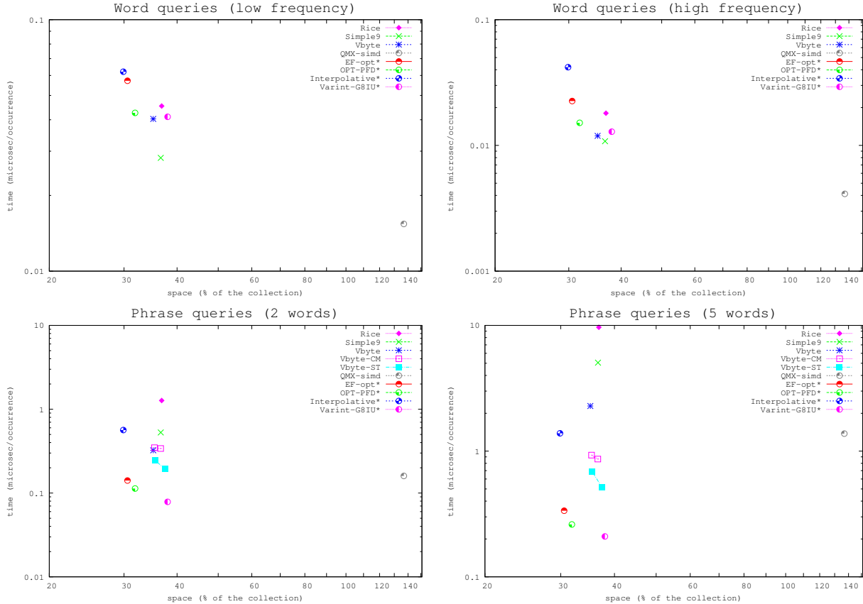
Figure 6: Space/time tradeoffs for traditional representations of positional indexes. Logscale.
