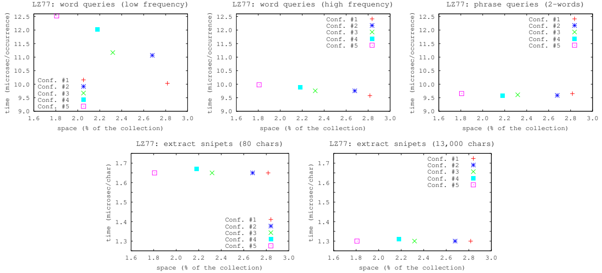
Figure 8: Space/time tradeoffs for different LZ77-index configurations.
