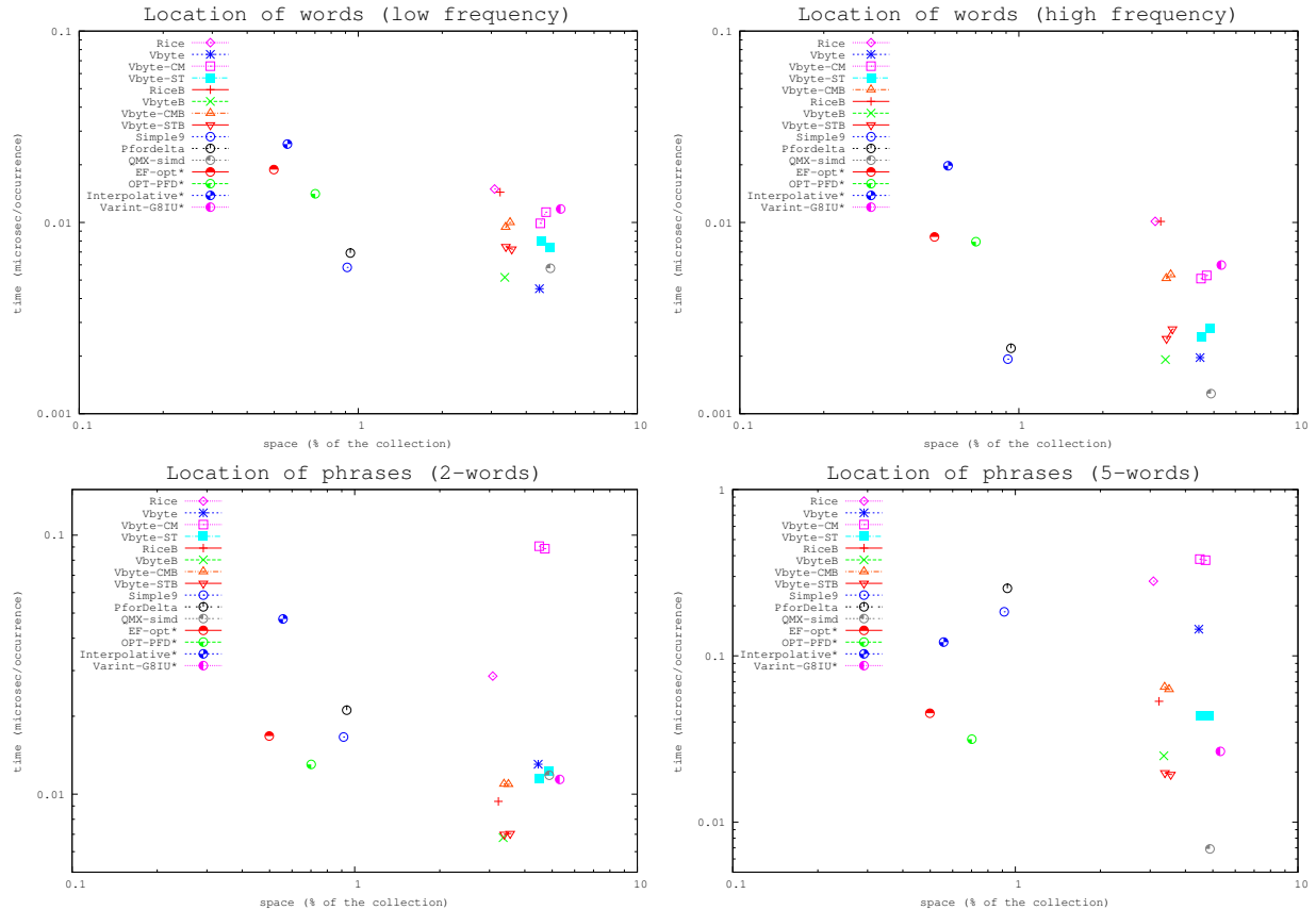
Figure 3: Space/time tradeoffs for non-positional indexes using traditional techniques. Logscale.
