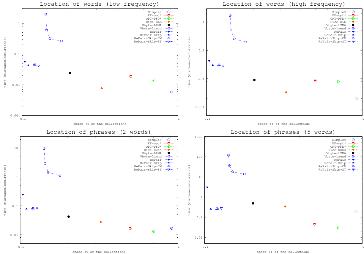
Figure 4: Space/time tradeoffs for non-positional indexes, comparing the best classical techniques with our new ones. Logscale.
