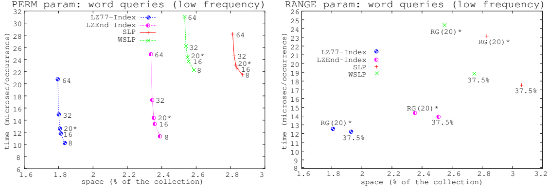
Figure 7: Space/time tradeoffs for fine tuning on perm (left plot) and range (right plot) parameters.
