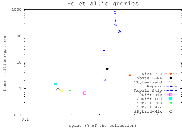
Figure 5: Space/time tradeoffs for our best non-positional indexes and those of He et al. Logscale.
