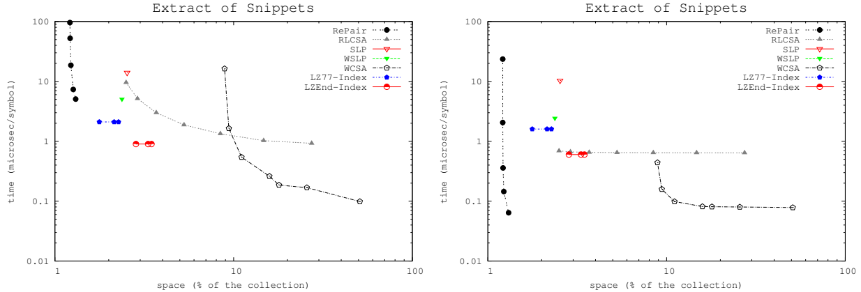
Figure 10: Space/time tradeoffs for extraction. Logscale.
