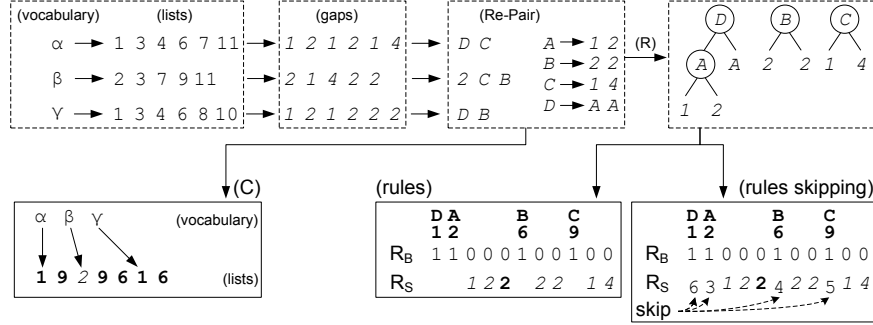
Figure 2: Example of inverted lists compressed with our Re-Pair-based method. Solid boxes enclose the data we finally keep. We include both variants of compressed rules with data aligned to the 1s in R_B (skipping) or not. Again, bold numbers (nonterminals) in the lists and R_S refer to positions in R_B , whereas slanted ones (terminals) refer to gap values.
