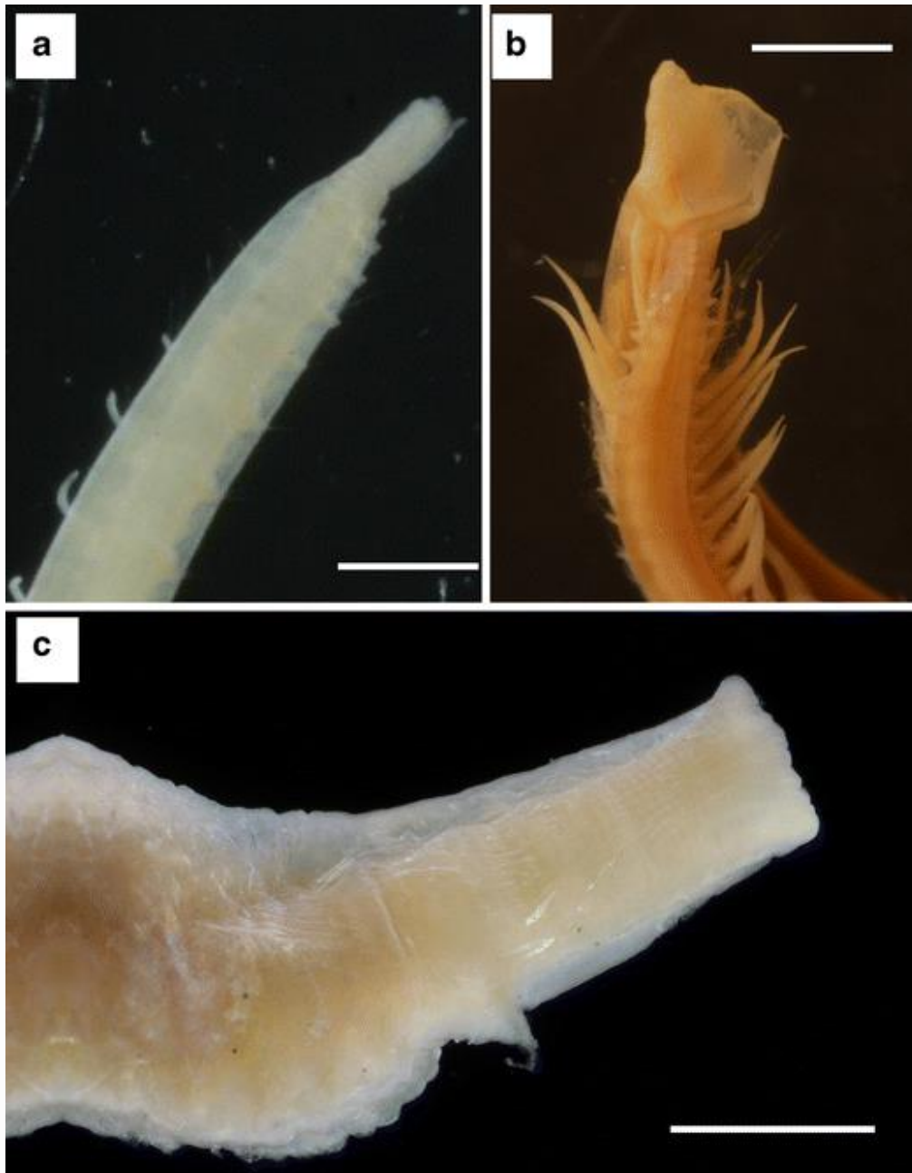
Fig. 10 Posterior body region in three North Atlantic-Arctic species of Ophelina not found in BIOICE samples. a O. groenlandica Støp-Bowitz, 1948 (holotype, SMNH T-7831). b O. norvegica Støp-Bowitz, 1945 (SMNH 11137). c O. nybelini Eliason, 1951 (syntype, GNHM Polych. 10999). Scale bars: (a) 0.5 mm; (b, c) 1 mm
