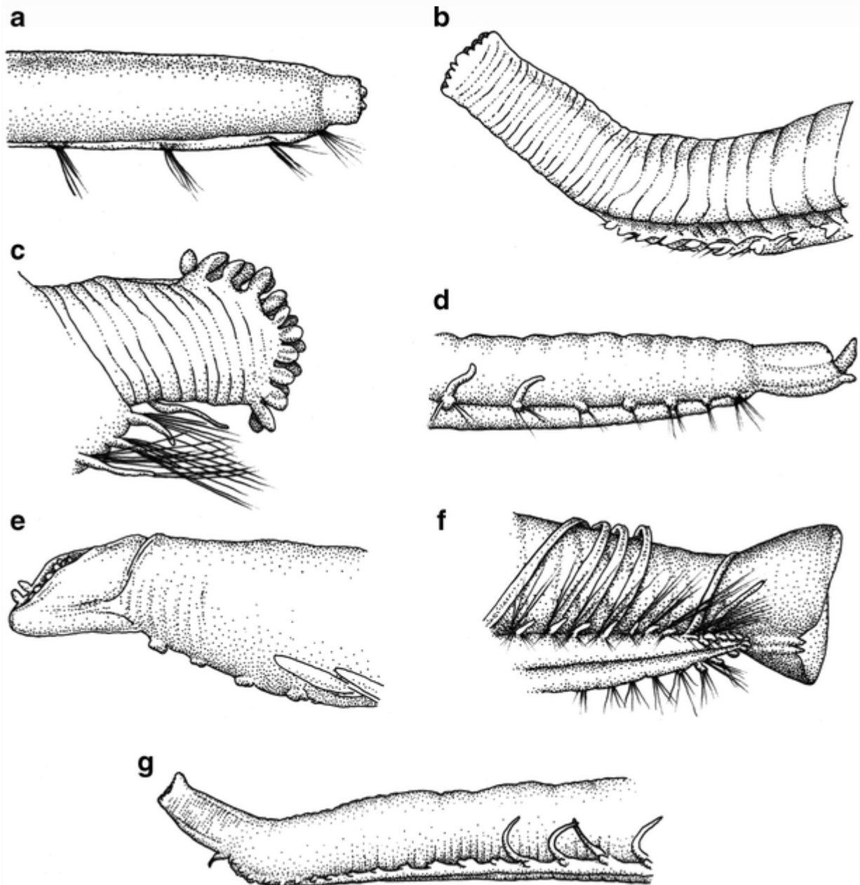
Fig. 9 Posterior body region in some Atlantic Ophelina species (redrawn from originals). a O. abbranchiata (from Støp-Bowitz 1948). b O. bowitzi sp. nov. (from Fauvel 1914, as A. arctica ). c O. delapidans longicephala (from Hartmann-Schröder 1977). d O. groenlandica (from Støp-Bowitz 1948). e O. helgolandica (from Augener 1912). f O. norvegica (from Støp-Bowitz 1945). g O. nybelini (from Eliason 1951)
