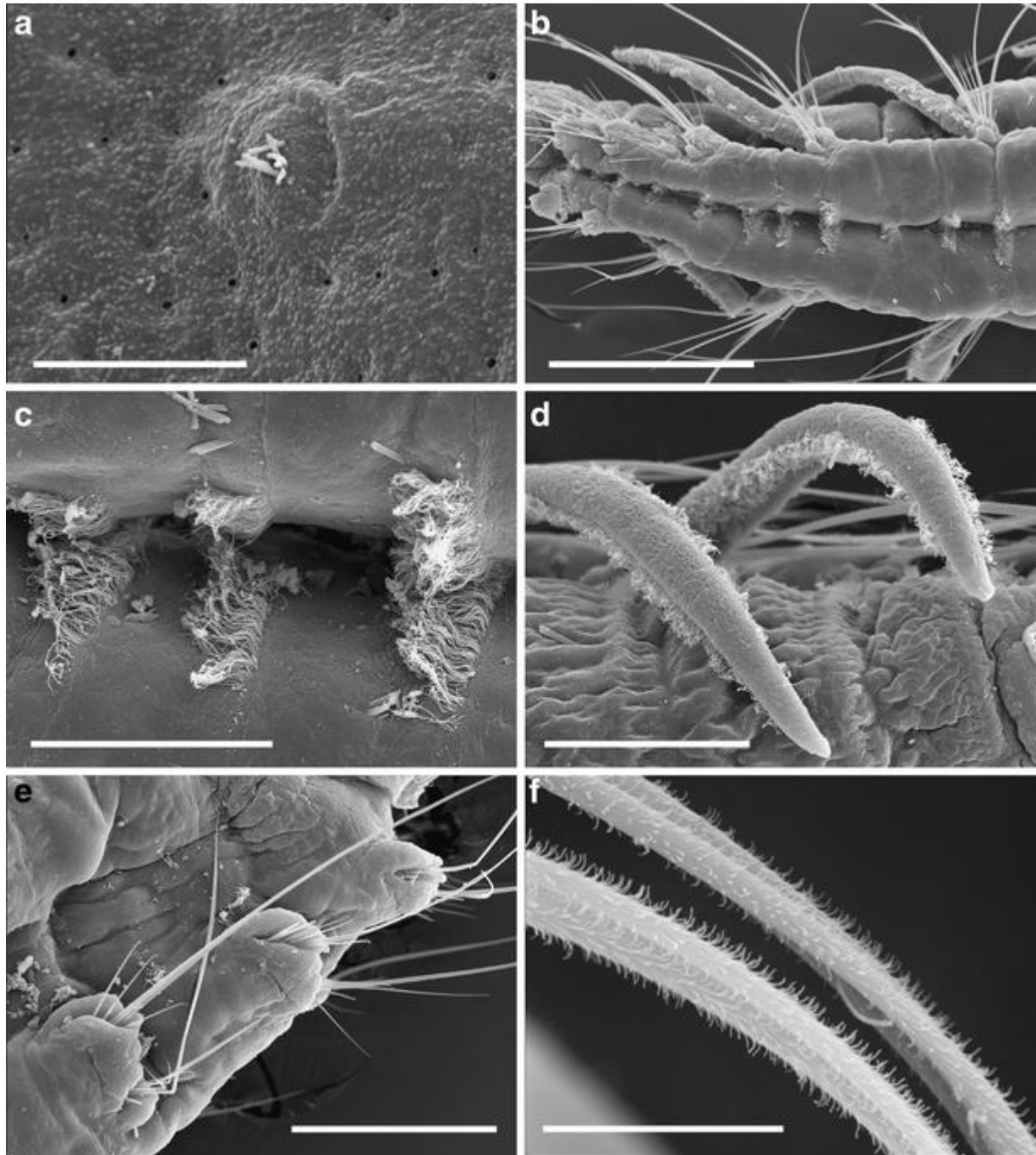
Fig. 7 Ophelina basicirra sp. nov. (paratypes, IMNH 24318, BIOICE sample 2303). a Cilia and pores on body surface. b Posterior end, ventral view. c Detail of ciliated ventral transverse bands. d Posterior body chaetigers. e Branchiae. f Detail of hirsute chaetae. Scale bars: ( a , f ) 10 \mu m; ( b ) 200 \mu m; ( c ) 50 \mu m; ( d ) 90 \mu m; ( e ) 100 \mu m
