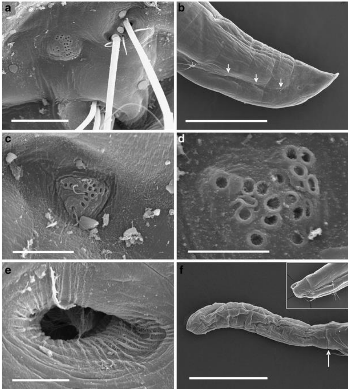
Fig. 4 Ophelina abranchiata (Støp-Bowitz) (IMNH 24328, BIOICE sample 3219). a Mid-body chaetiger. b Anterior end, lateral view; arrows mark positions of lateral organs of first achaetigerous segments. c Lateral organ of an achaetigerous anterior segment. d Detail of lateral organ. e Nuchal organ. f Anal tube; arrow shows breakline; insert: detail of posterior end without anal tube. Scale bars: (a) 20 \mu\text{m} ; (b) 600 \mu\text{m} ; (c, e) 10 \mu\text{m} ; (d) 5 \mu\text{m} ; (f) 900 \mu\text{m}
