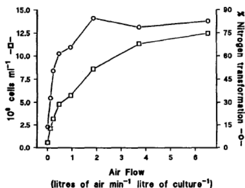
Fig. 1. Stationary phase cell density (10 6 cells ml -1 ) and percentage of conversion of nitrate into protein in mass cultures of D. tertiolecta with different air flows. Values are the averages of two replicates.
