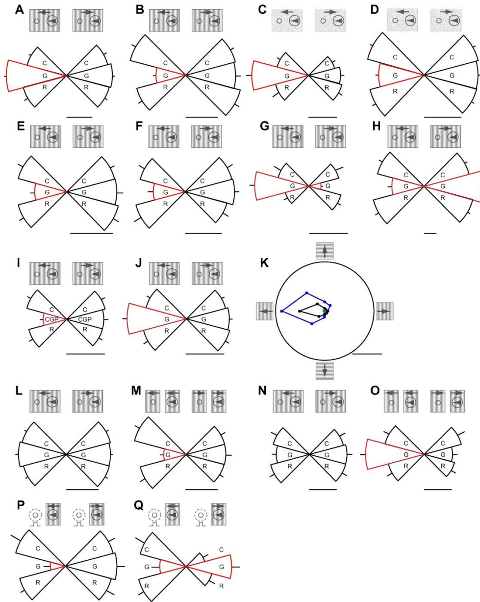
Fig. 2. Inactivation of an MT direction column can evoke clear and reversible changes in the responses of LGN cells. (A, B) The histograms document the responses of two typical LGN cell examples to a large patch of grating drifting in the preferred (left) and non-preferred (right) directions of the MT inactivation site, before (C), during (G) and after cessation of (R) GABA application in MT. Red shading indicates that there was a significant difference ( P < 0.05 , paired t -test, see Experimental procedures) between the responses observed during control and MT inactivation conditions. Error bars 1 SE. Scale bars = 10 s/s. Here, and in all subsequent panels and figures, the iconic representation of the MT and LGN cell receptive field locations and stimulus configuration drawn above the records are for illustrative purposes only, and not to scale. (C, D) The histograms document the responses of two typical LGN cell examples to a large patch of texture drifting in the preferred (left) and non-preferred (right) directions of the MT inactivation sites before (C), during (G) and after cessation of (R) iontophoretic application of GABA in MT. Error bars 1 SE. Scale bars = 20 s/s. (E, F) Repeatability of influence of MT inactivation over time. The histograms document the responses of an LGN cell to a patch of grating drifting in the preferred (left) and opposite directions of motion (right) of the MT inactivation site, before (C), during (G) and after cessation of (R) GABA application in MT. The histogram in (E) shows the responses during the initial application of GABA in MT and that in (F) the responses observed during a subsequent test cycle recorded over an hour later. Scale bar = 10 s/s. (G, H) Reciprocal effects of inactivation of an MT direction column on LGN cell responses to the MT site preferred direction of motion and its reverse. The histograms document the responses of two LGN cells to a patch of grating drifting in the preferred (left) and opposite directions of motion (right) of the MT inactivation site, before (C), during (G) and after cessation of (R) GABA application in MT. Scale bar = 15 s/s. (I-K) Iontophoretic application of GABA and the GABA B receptor antagonist CGP 55845 in MT evoke opposite effects on the responses of LGN cells. The histograms in (I) document the responses of an LGN cell to a patch of grating drifting in the preferred (left) and opposite directions of motion (right) of the MT locus, before (C), during (CGP) and after cessation of (R) CGP 55845 application in MT. The histograms in (J) shows the responses of the same cell observed during GABA application in MT. Scale bar = 15 s/s. During CGP application in MT, the LGN cell's response to the stimulus moving in the MT preferred direction of motion was significantly reduced whereas it was significantly increased during GABA iontophoresis in MT. This reciprocal pattern of effect held across our sample ( n = 5 ) of cells tested with both GABA and CGP 55845, with a significant negative correlation in the normalized response change observed in the two conditions ( R = -0.9 ,
