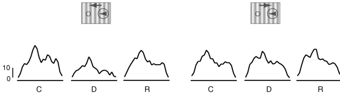
Fig. 3. Example documenting the effect of inactivation of an MT direction column on the responses of an LGN cell plotted as peri-stimulus time histograms (PSTHs). The wrapped PSTHs document the responses of the cell illustrated in Fig. 2B. Responses to the preferred (left) and non-preferred (right) directions of motion of the MT inactivation site are shown before (C), during (D) and following recovery from (R) GABA application in MT. Scale bars = 10 s/s. Fifteen milliseconds bins, traces smoothed with a Gaussian window at 1.5 times the bin width.
