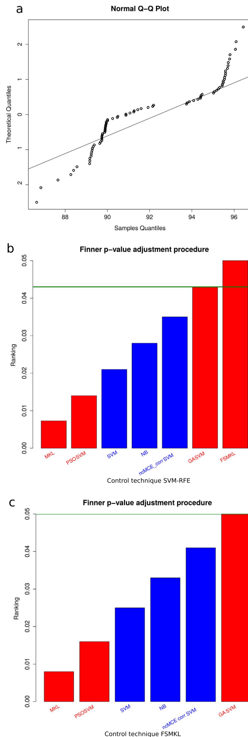
Figure 4. Best model determination. (a) Q-Q plot of observed versus expected values. (b) Finner p-value adjustment post hoc procedure. Control technique: SVM-RFE. (c) Finner p-value adjustment post hoc procedure. Control technique: FSMKL. Machine Learning techniques with Feature Selection are in red, without Feature Selection are in blue.
